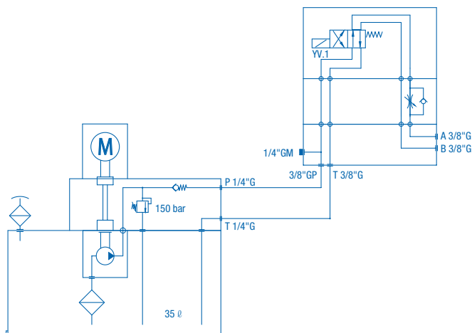
SCHEMA IDRAULICO / HYDRAULIC SCHEMATIC
