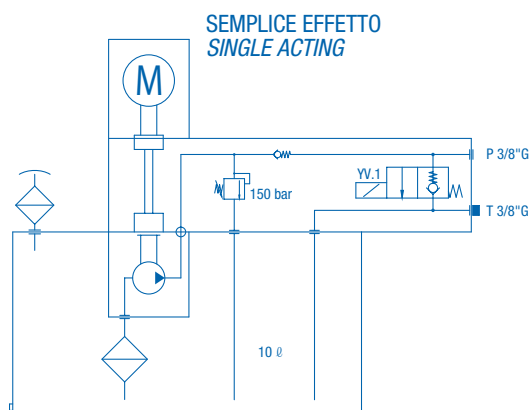
SCHEMA IDRAULICO / HYDRAULIC SCHEMATIC
