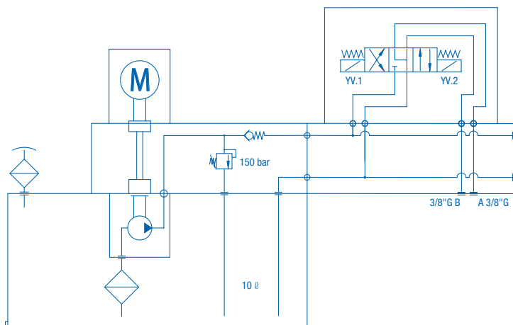
SCHEMA IDRAULICO / HYDRAULIC SCHEMATIC
